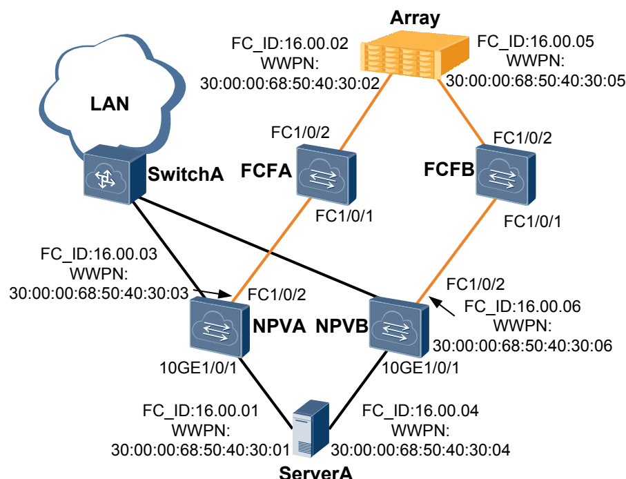
Figure 14-5 FCF+NPV Networking
