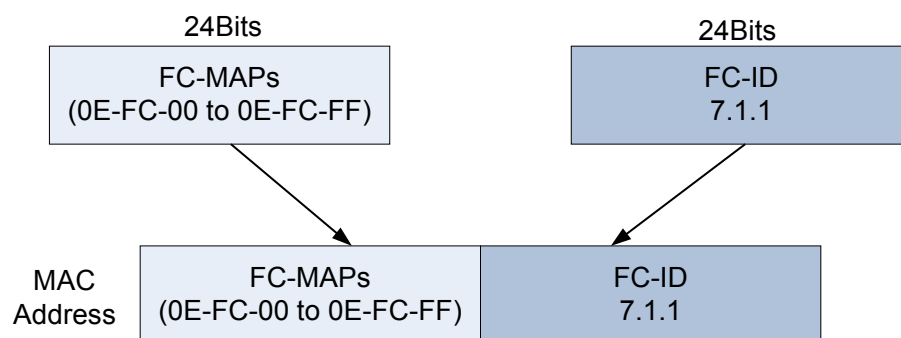
Figure 4-7 FPMA format
