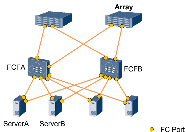
Figure 5-3 Typical FCF networking (FC interface)
