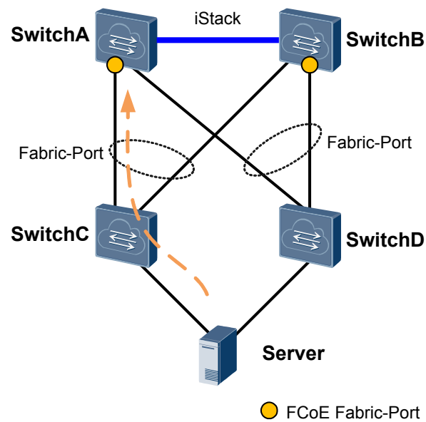
Figure 10-2 SVF networking
