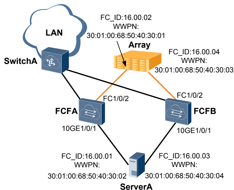
Figure 14-3 FCF networking
