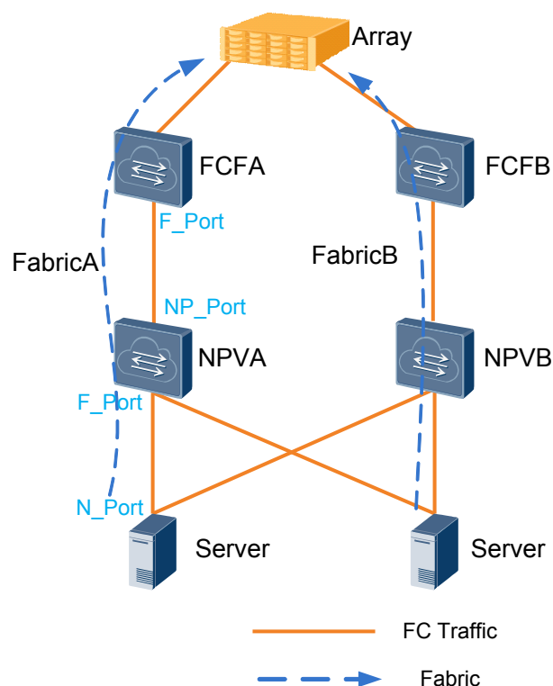
Figure 3-1 FC networking
