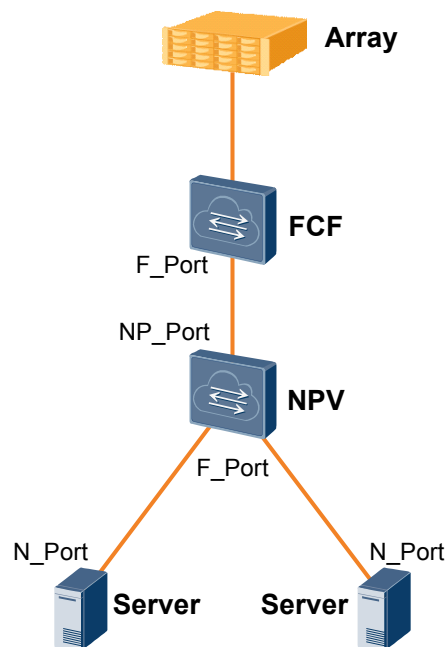
Figure 3-7 NPV networking
