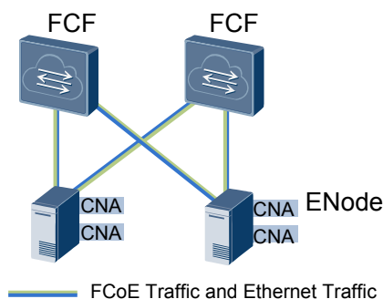
Figure 4-8 Direct connection
