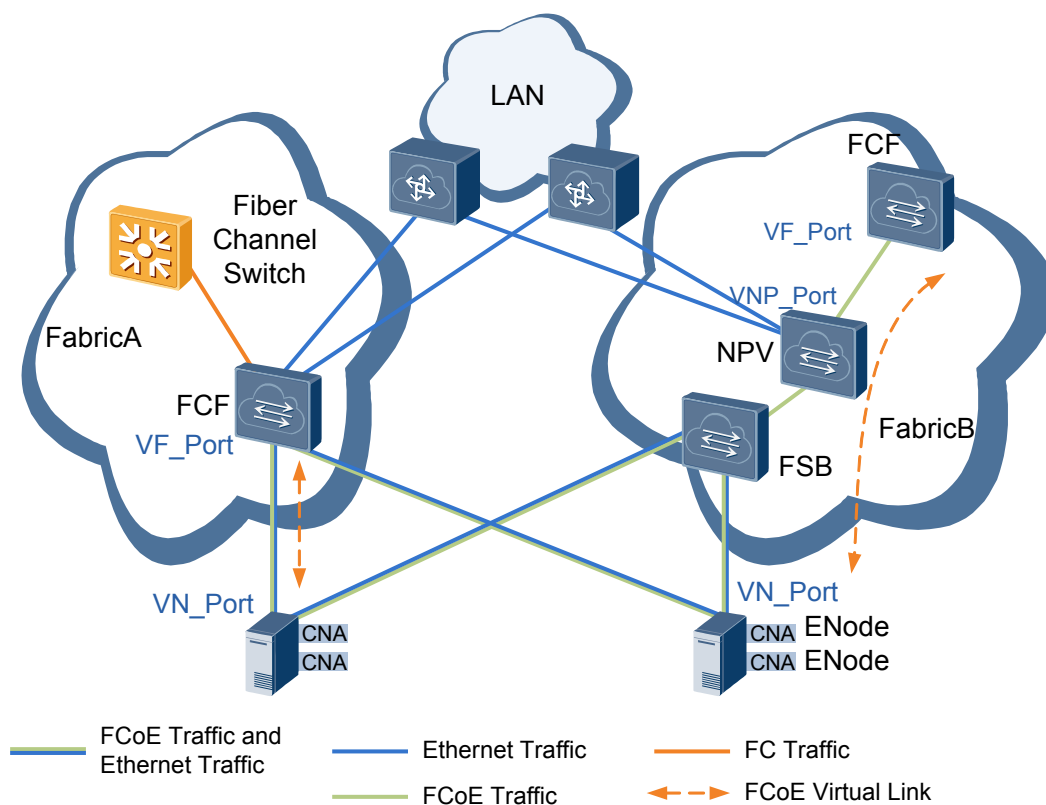
Figure 4-1 FCoE networking
