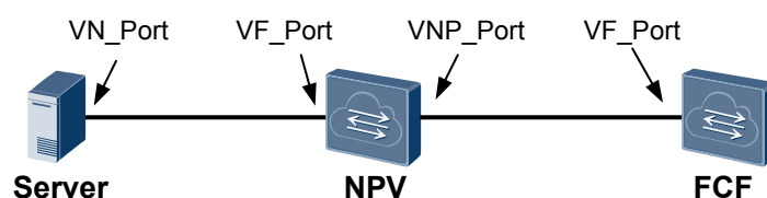
Figure 4-3 Interface roles
