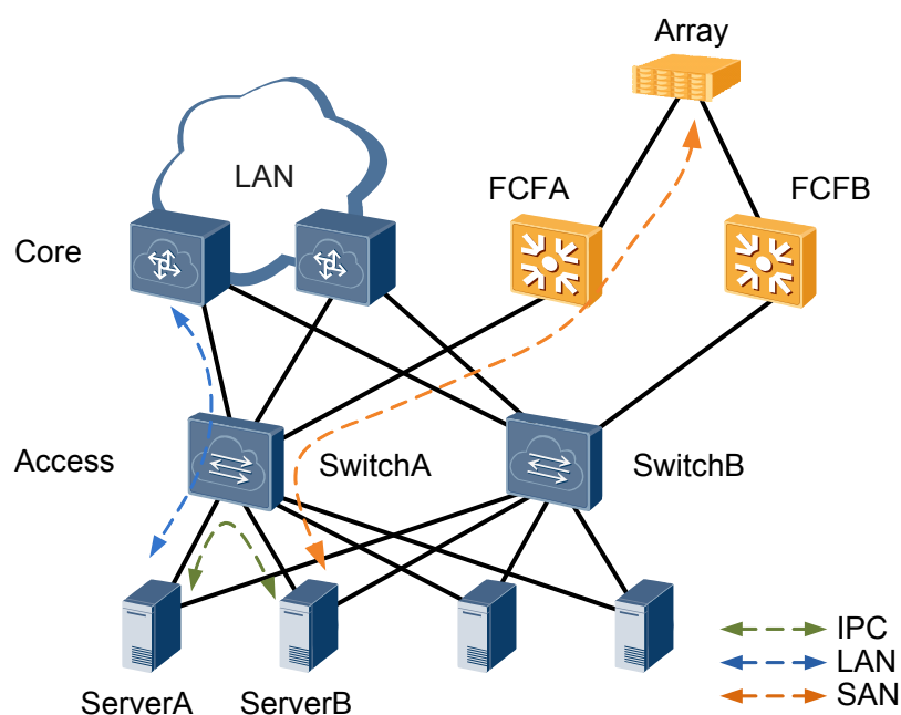
Figure 17-1 FSB networking
