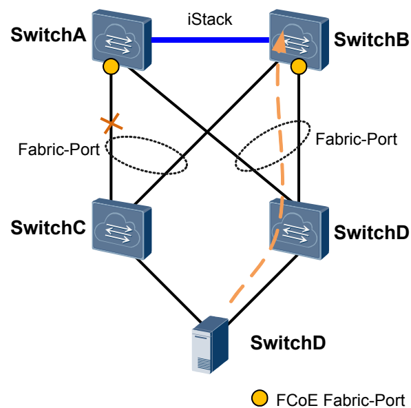
Figure 10-3 SVF networking
