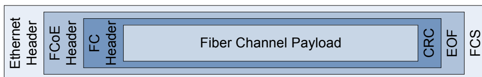
Figure 4-5 FCoE frame encapsulation
