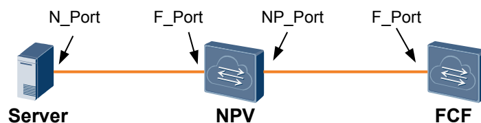
Figure 3-4 Interface role
