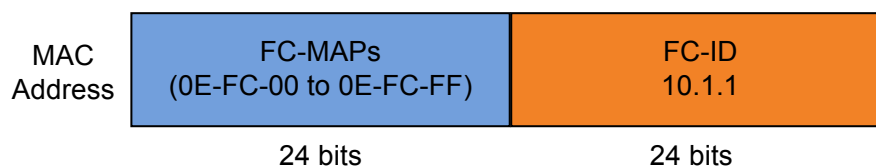
Figure 3-3 FPMA
