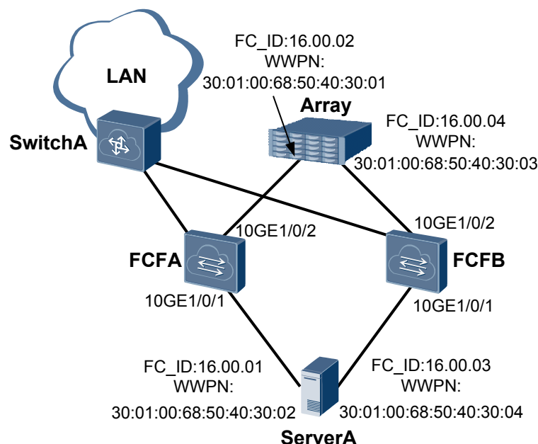
Figure 14-2 FCF networking
