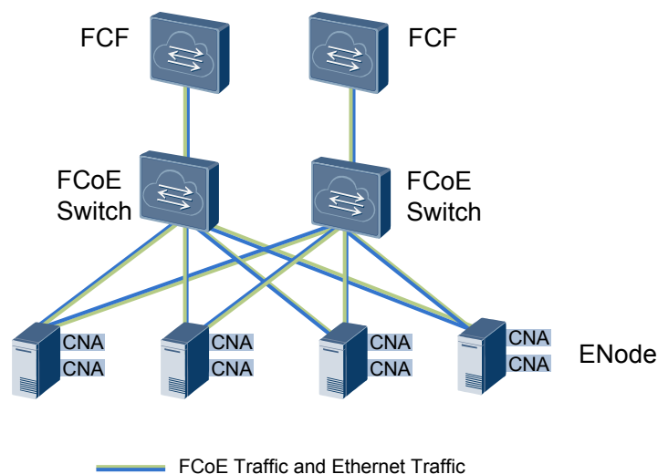
Figure 4-9 Remote connection
