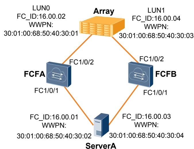
Figure 14-1 FCF networking
